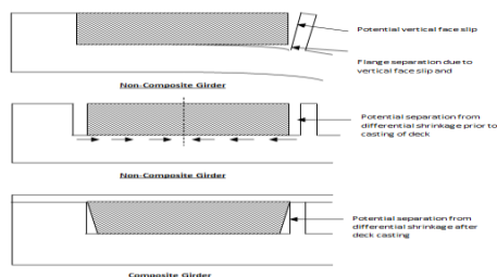
Figure 7 – Potential Separation from Differential Shrinkage
