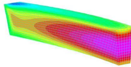
Figure 11 – Shear Stress Distribution (Infill Diaphragm)
