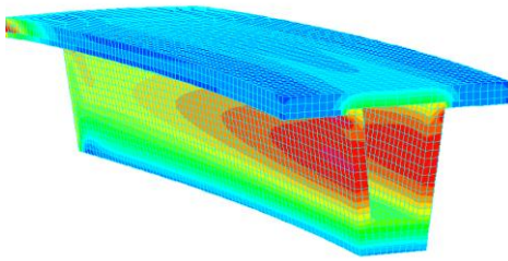
Figure 10 – Shear Stress Distribution (Composite Super-T)
