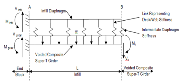
Figure 8 – Free Body Diagram of Vierendeel Truss Mechanism
