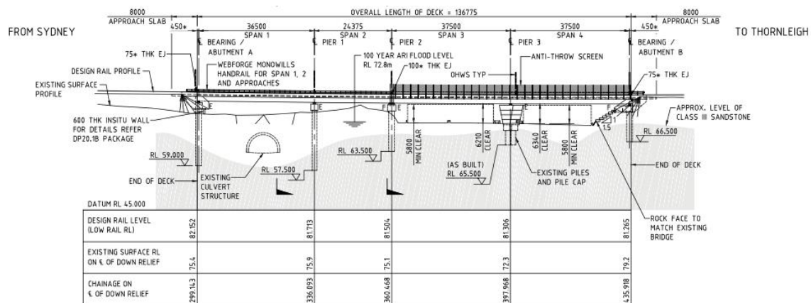
Figure 1 – Bridge Elevation
