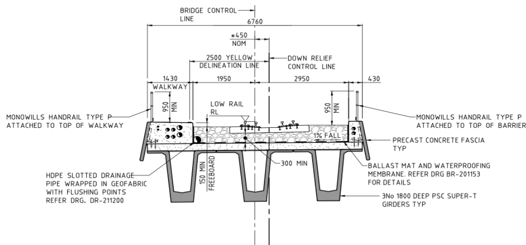
Figure 2 – Bridge Typical Cross Section
