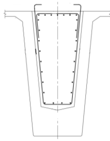
Figure 5 – Infill Diaphragm
