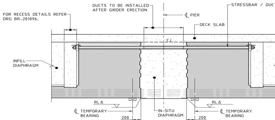
Figure 4 – Continuity Joint Detail
