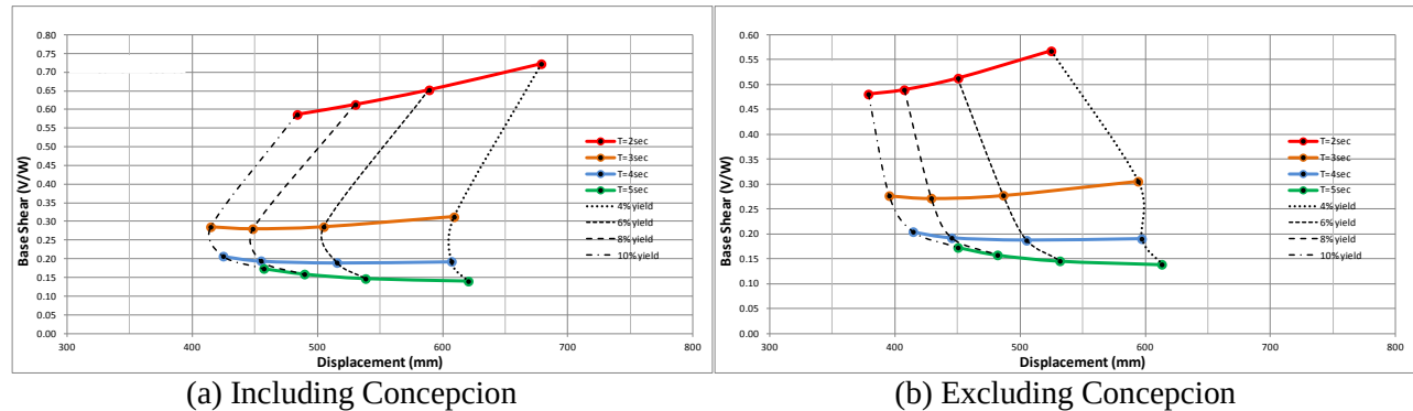
Fig. 11. ADRS for all records for three earthquakes, single-scale factor, including and excluding Concepcion
