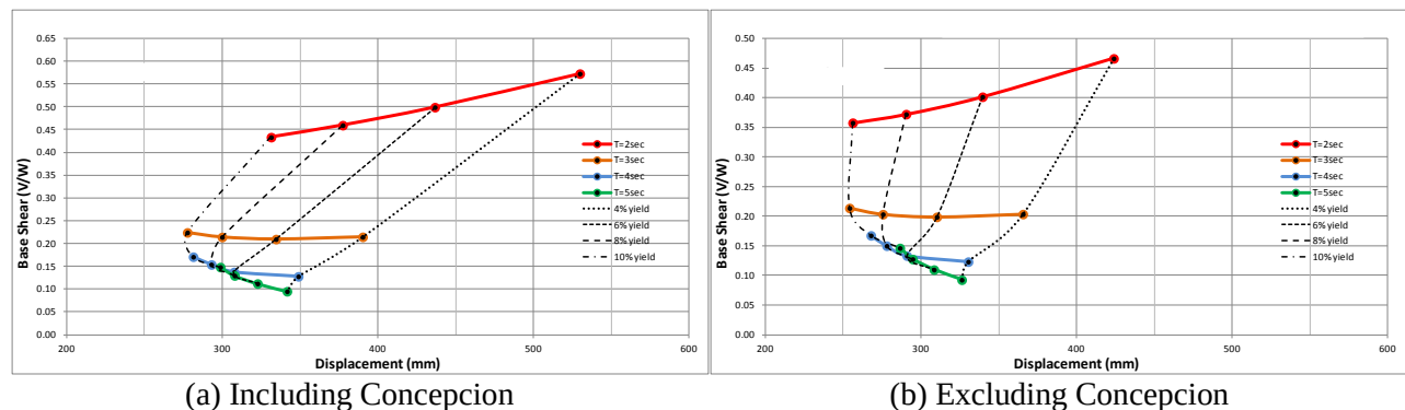
Fig. 12. ADRS for all records for three earthquakes, frequency scaled, including and excluding Concepcion
