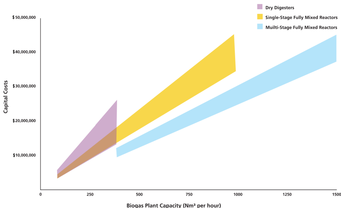
Figure 8: Capital cost ($NZD) vs biogas plant capacity (Nm³/h) for dry digesters, single-stage fully mixed reactors and multi-stage fully mixed reactors
